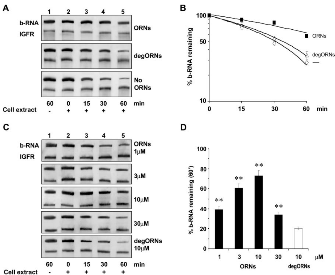
Fig. 2. Inhibition of b-RNA degradation by ORNs in vitro. A, the mixture of the three ORNs or the degORNs, total dose 10 \mu M, was added to the degradation mixture containing the total extract from the DOHH2 lymphoma cells, b-RNA (530 nt), and IGFR-RNA (350 nt). Incubation times with and without cell extract are indicated. B, time course of decay of b-RNA estimated by laser densitometry of the gel bands. Mean \pm S.D. from three assays. C, dose-response assay of ORNs, experimental conditions as in A. D, histograms of C (incubation for 60 min at the indicated doses) obtained by densitometry (mean \pm S.D., n = 3 ). Statistical significance was calculated versus degORN 10 \mu M treatment.
